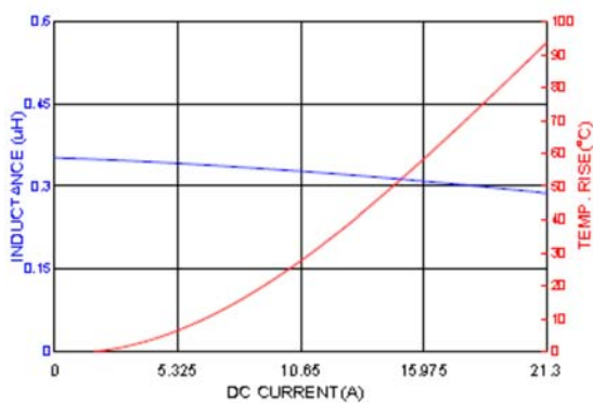
HMPL0502HP-R33
