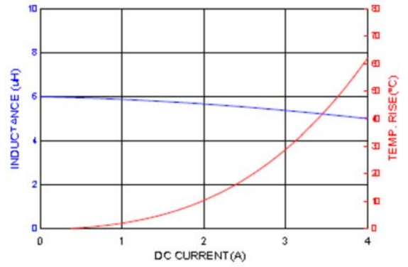
HMPL0502HP-5R6
